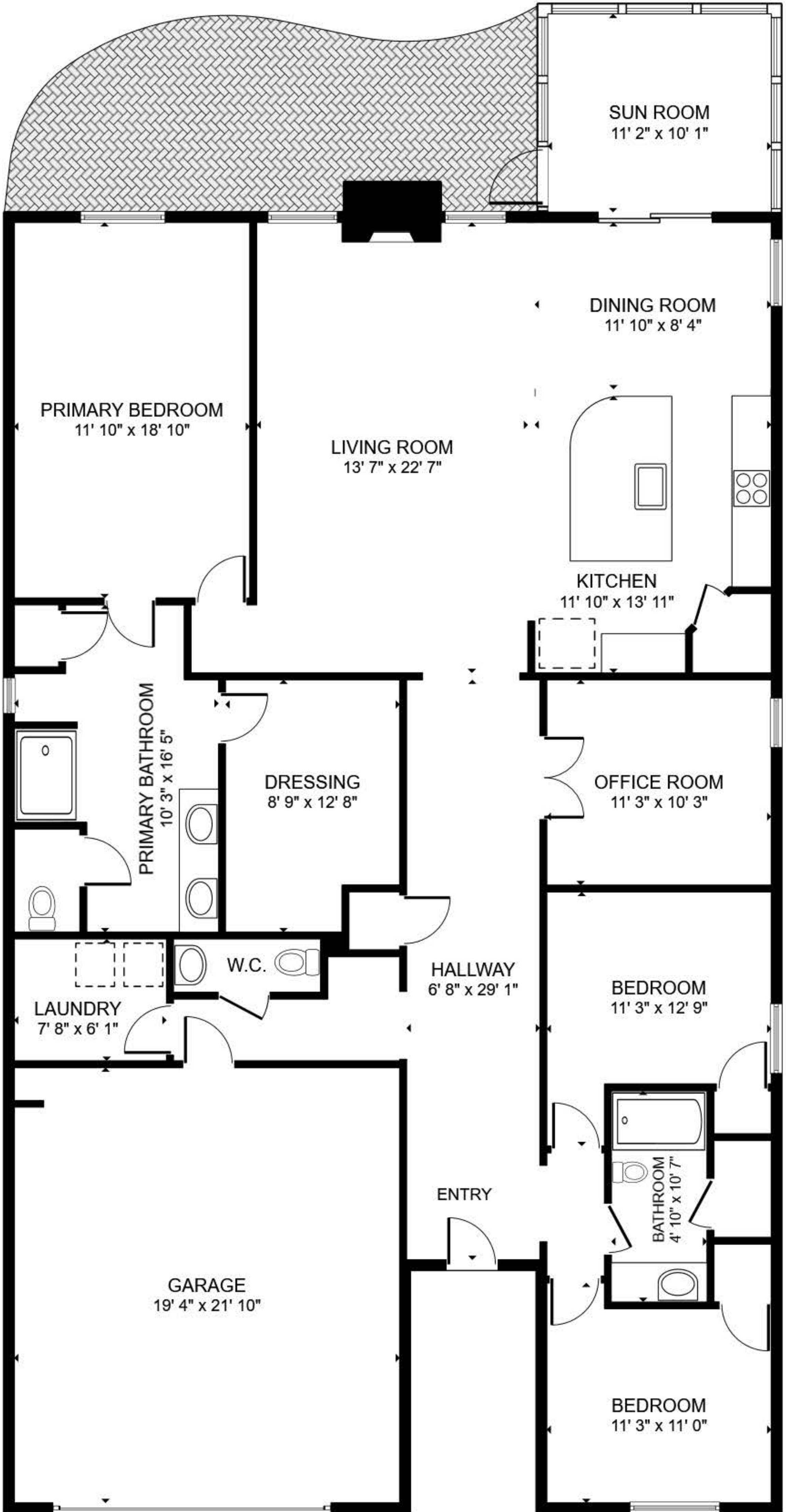
FLOOR PLAN
